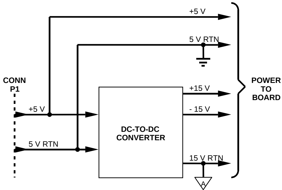
Figure 1-5 Power Converter
