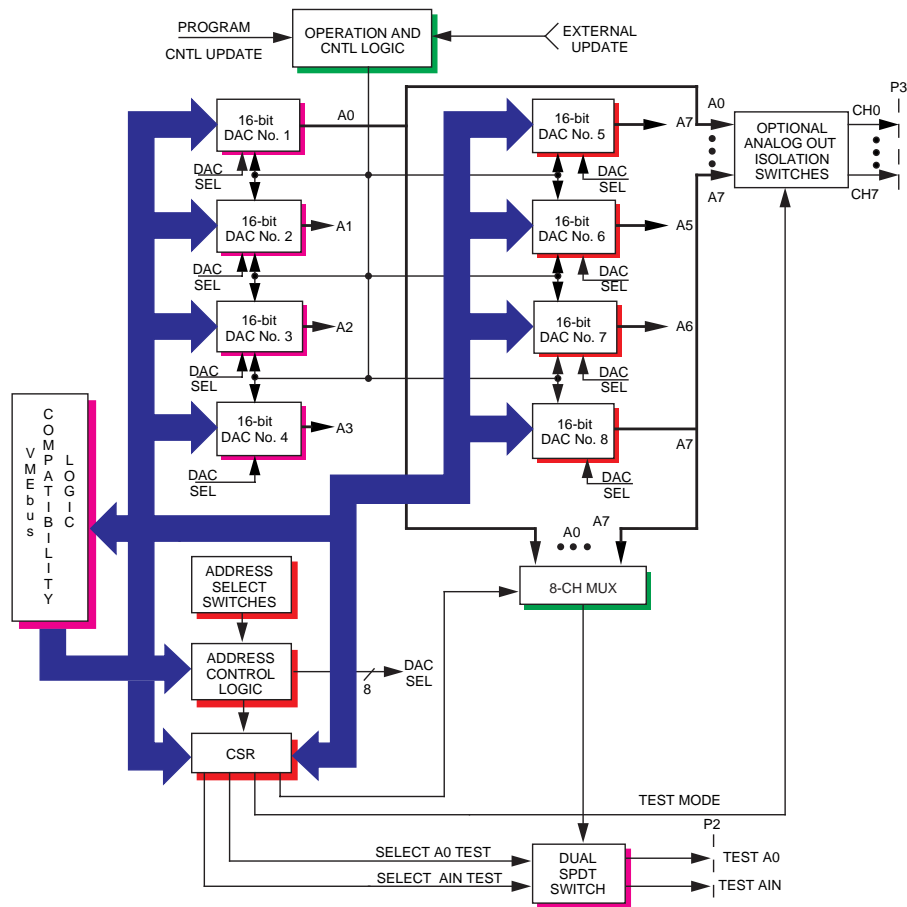
Figure 1. VMIVME-4116 Board Functional Block Diagram
