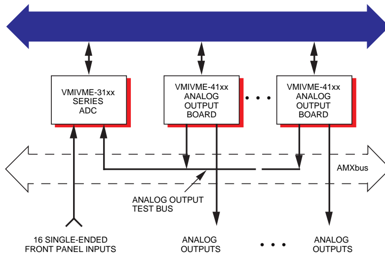
Figure 1. VMIVME-4116 Board Functional Block Diagram
