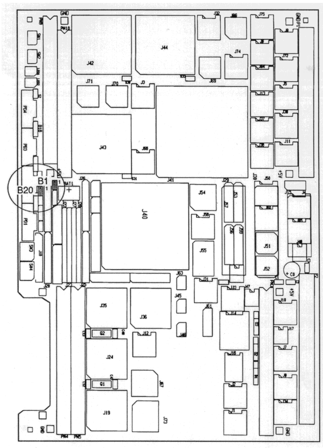
Figure 3-5: Location Diagram of the Backup Supply Jumperfield B1 and B20
