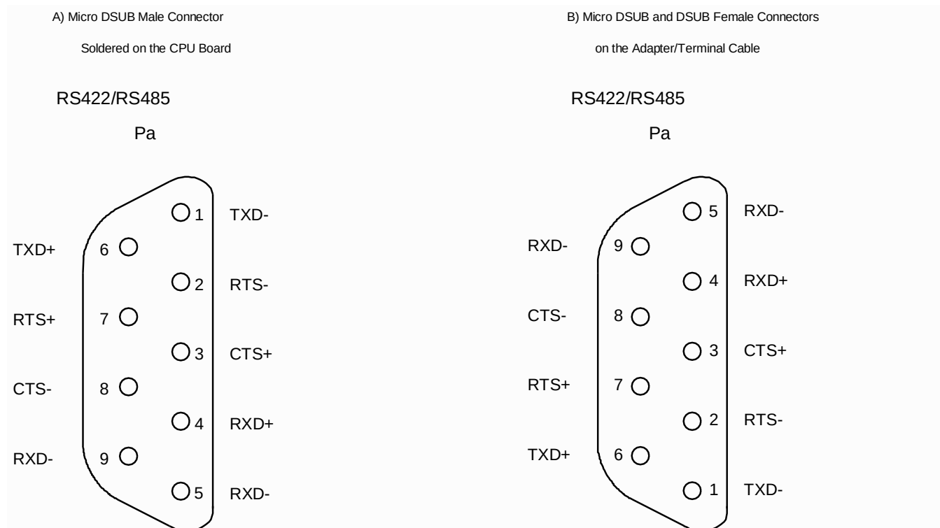
Figure 3-14: RS422/RS485 Pinout of the Micro D-Sub and D-Sub Connectors
