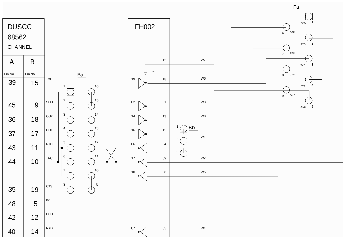
Figure 3-17: Connection Between DUSCC2 and D-Sub Connector for RS232
